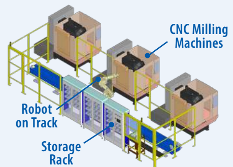
Milling Robot-on-Track Cell (MRTC)
